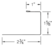
③⑨ ABS Starter "J" (ABSSJcc)
