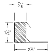
①② ABS Vented "Z" Closure (ABSZVcc)
