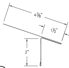
③⑤ ABS Residential Eave (ABSREcc)
