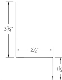
④④ ABS Sidewall (ABSSWcc)
