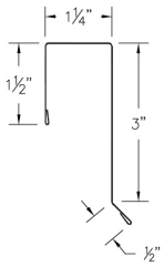
④⑤ ABS Rake Trim (ABSRtcc)
