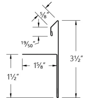
⑤① ABS Slim Line Rake (ABSSLRcc)
