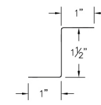
③⑧ ABS Metal "Z" Closure (ABSZcc)
