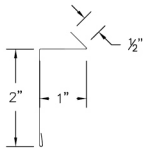
④③ ABS Counter Flashing (ABSCFcc)
