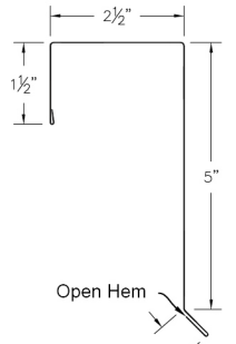
④① ABS Gable Flasing (ABSGFcc)
