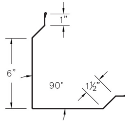
(56) PBR Outside Corner (PBRRCcc)
