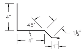
(52) PBR Universal Sidewall (PBRSWcc)
