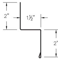
(53) PBR Double Angle (PBRDAcc)
