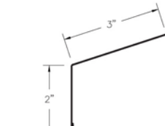
㉑ Gutter Apron (GAcc)
