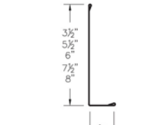
⑩ Post/Fascia Trim (PTcc)
