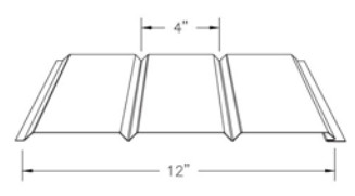
⑷ 12" Soffit (Solid or Vented)
