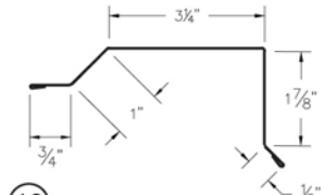
⑱ Residential Rake (RRcc)
