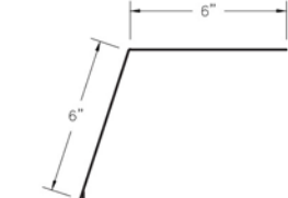
⑵ Gambrel Trim (GTcc)
