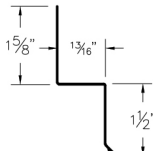
⑦ Double Angle (DAcc)
