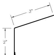
㉑ Gutter Apron (GAcc)
