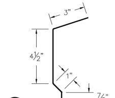
④ Fascia Trim (FTcc)
