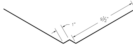
⑲ Formed Valley (WVcc)
