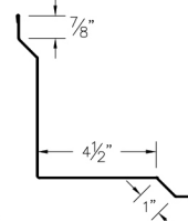
⑬ Inside Corner (ICcc)
