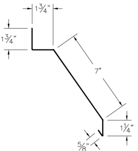
⑮ Face Mount Track Cover (CTcc)
