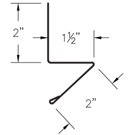
54 PBR Base Angle (PBRBAcc)
