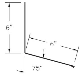
11 Universal Endwall (PBREWcc)
