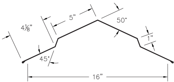
34 20" Ridge Cap (CP20cc)
