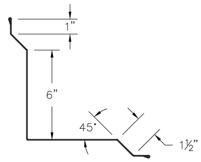
58 PBR Inside Corner (PBRICcc)
