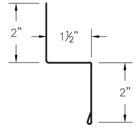
53 PBR Double Angle (PBRDAcc)
