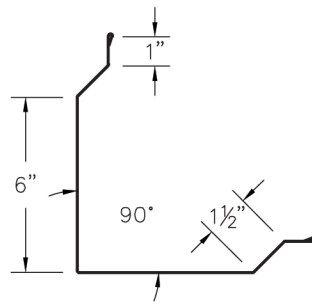
56 PBR Outside Corner (PBRRCcc)
