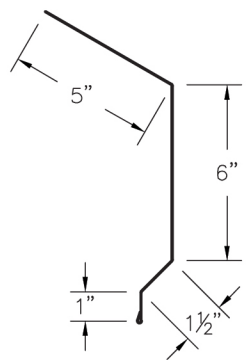
57 PBR Fascia Trim (PBRFTcc)
